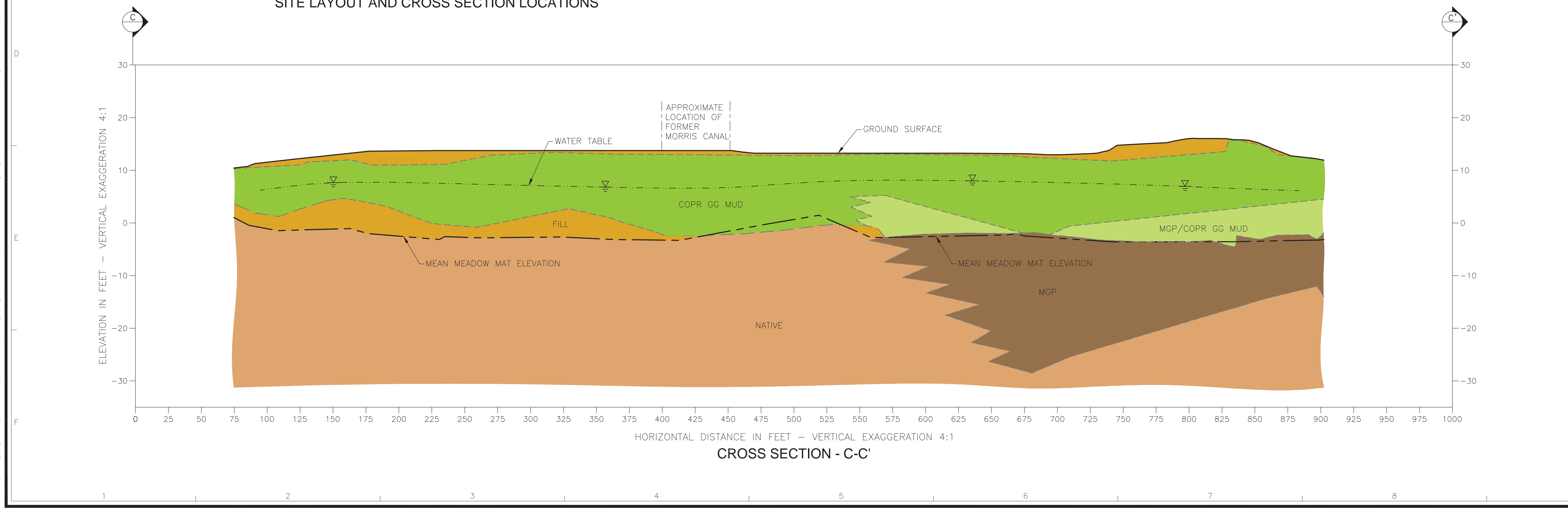
SITE LAYOUT AND CROSS SECTION LOCATIONS
