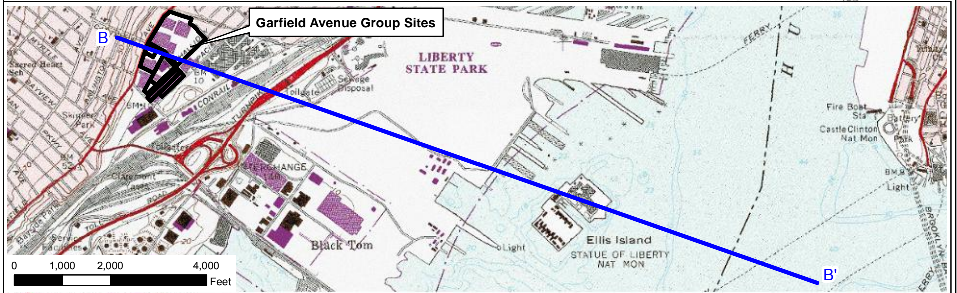
FIGURE 3-2 REGIONAL SURFICIAL GEOLOGY CROSS-SECTION
