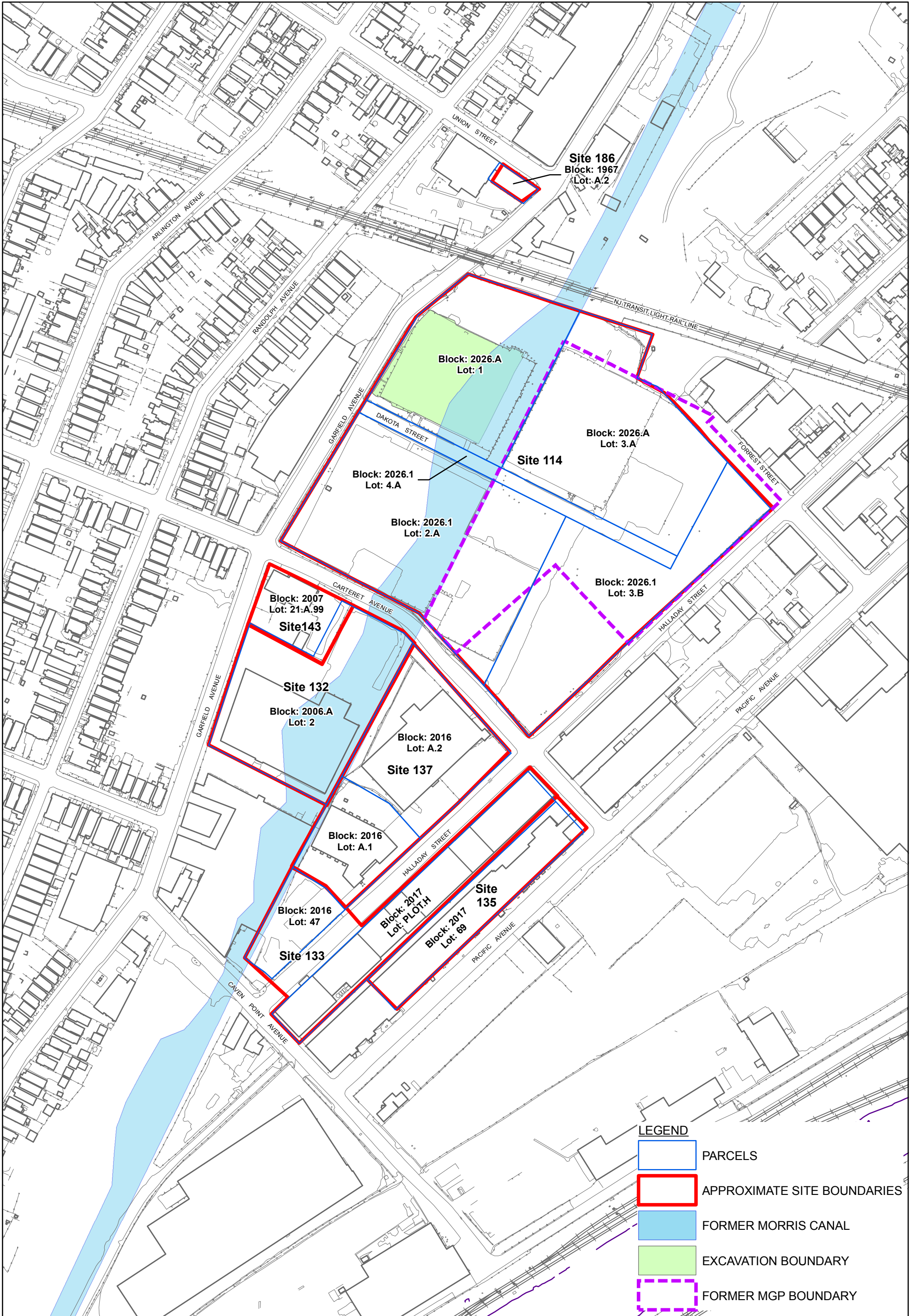
FIGURE 1-2 SITE PLAN
