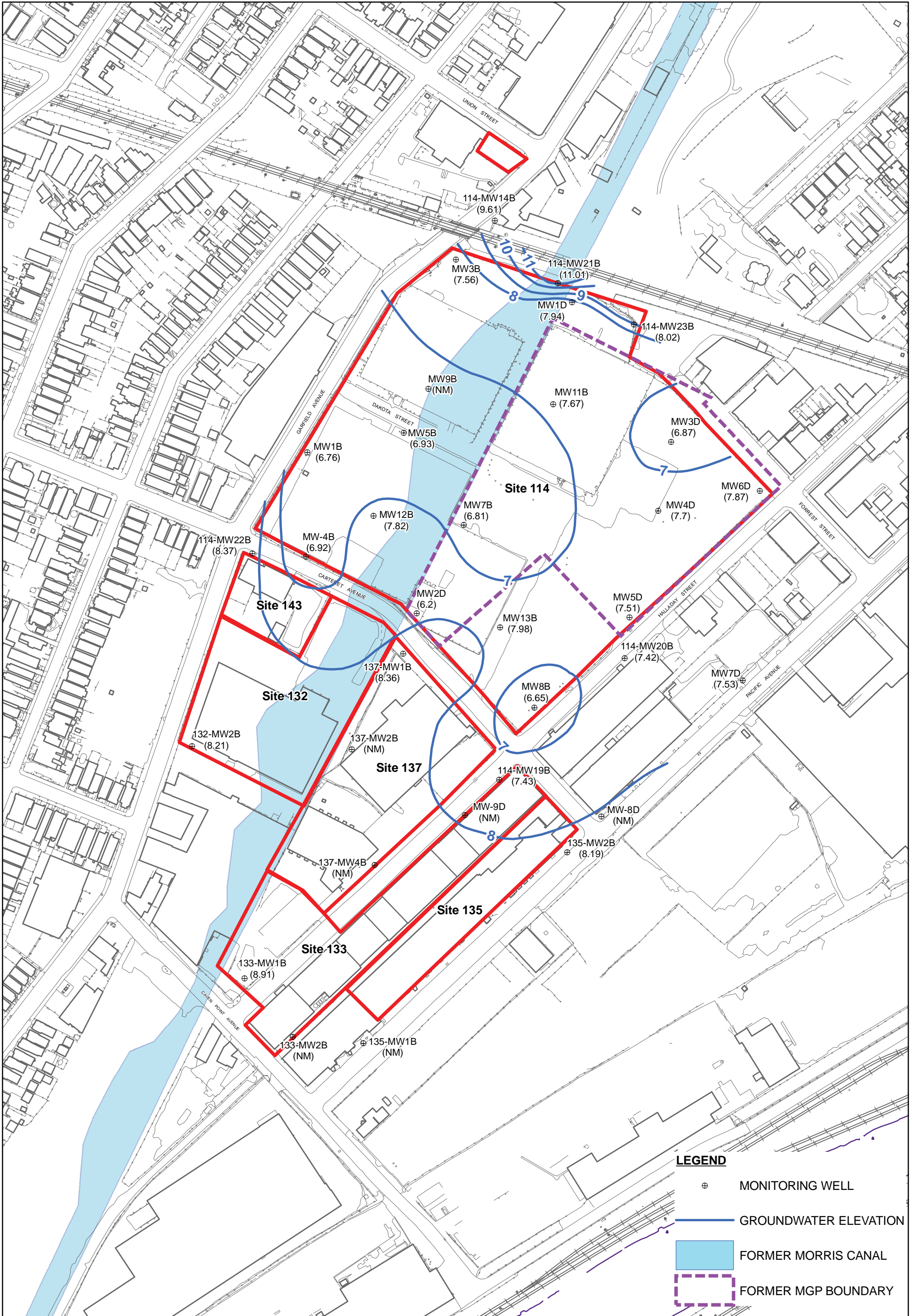
FIGURE 3-10 MAY 2011 GROUNDWATER CONTOUR MAP INTERMEDIATE MONITORING WELLS
