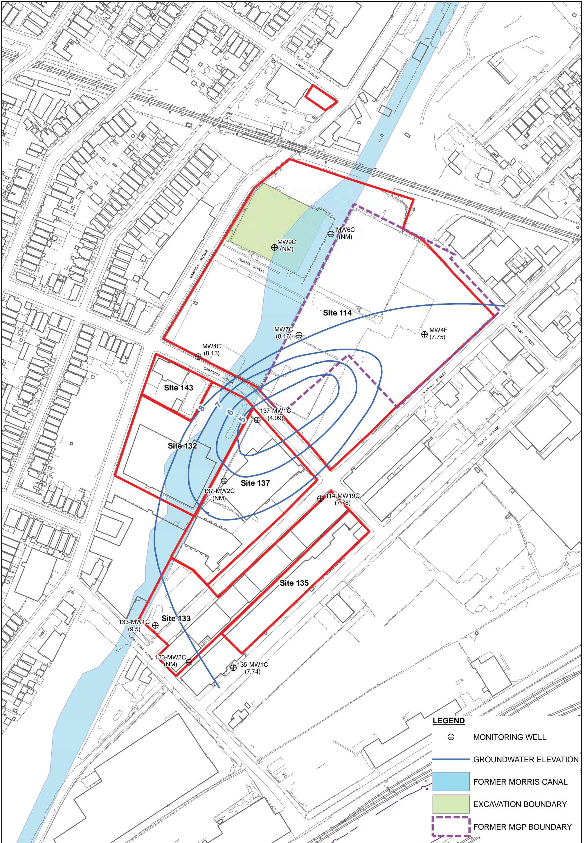
FIGURE 3-11 MAY 2011 GROUNDWATER CONTOUR MAP DEEP MONITORING WELLS
