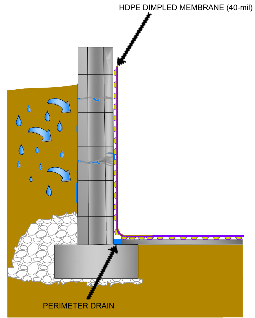
BOILER ROOM BASEMENT HDPE DIMPLED MEMBRANE SECTION A-A' NTS
