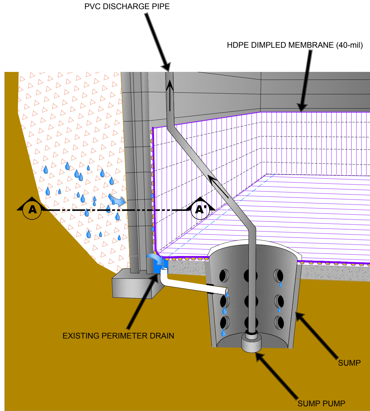
BOILER ROOM BASEMENT HDPE DIMPLED MEMBRANE ISOMETRIC VIEW NTS
