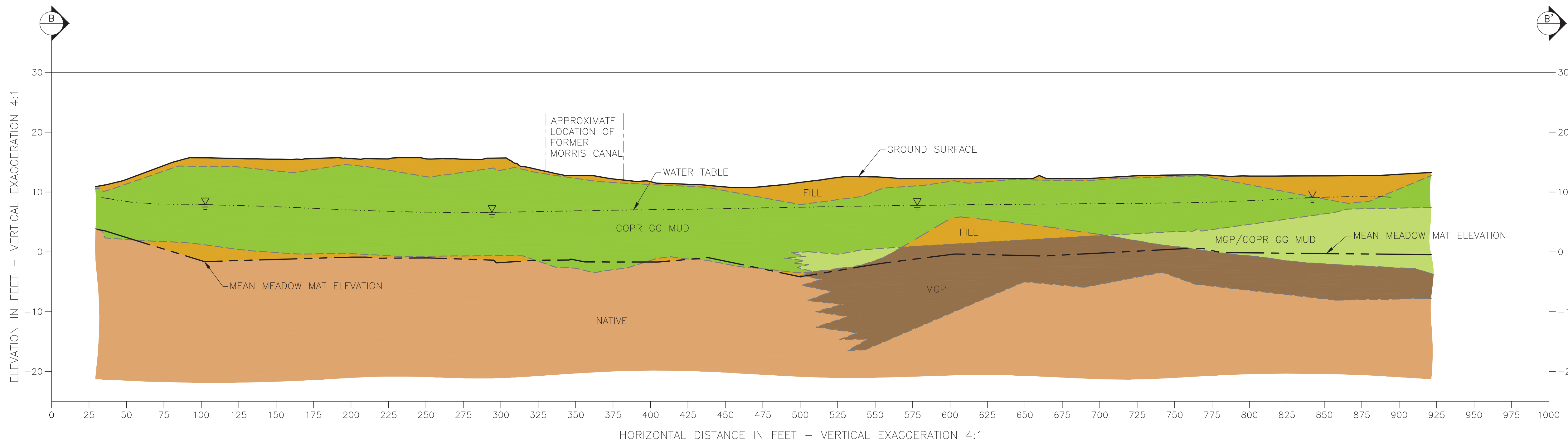
CROSS SECTION - B-B'
